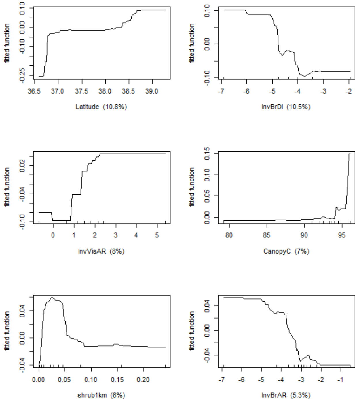
Fig. 43. Partial dependence plots for the six most influential variables that predict migrant density for all nocturnal landbird species included in the Period 3 analysis. Rug plots located at the bottom of plots show the distribution of data, in deciles, for the X-axis variable. Relative influence is in parentheses. See Table 1 for predictor variable descriptions.
