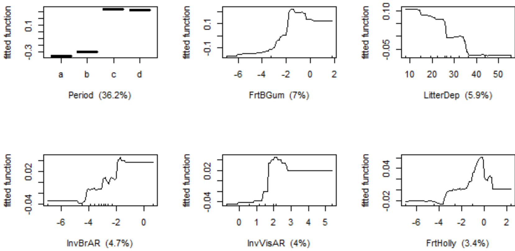
Fig. 41. Partial dependence plots for the six most influential variables that predict (Yellow-shafted) Northern Flicker density. Rug plots located at the bottom of plots show the distribution of data, in deciles, for the X-axis variable. Relative influence is in parentheses. See Table 1 for predictor variable descriptions.
